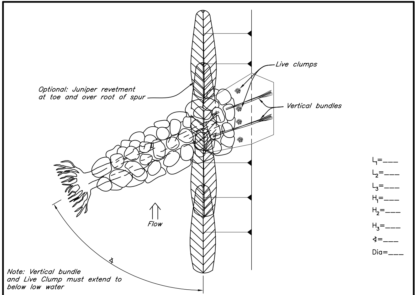
ROCK BARB WITH ROOT WAD (PLAN) N.T.S.
