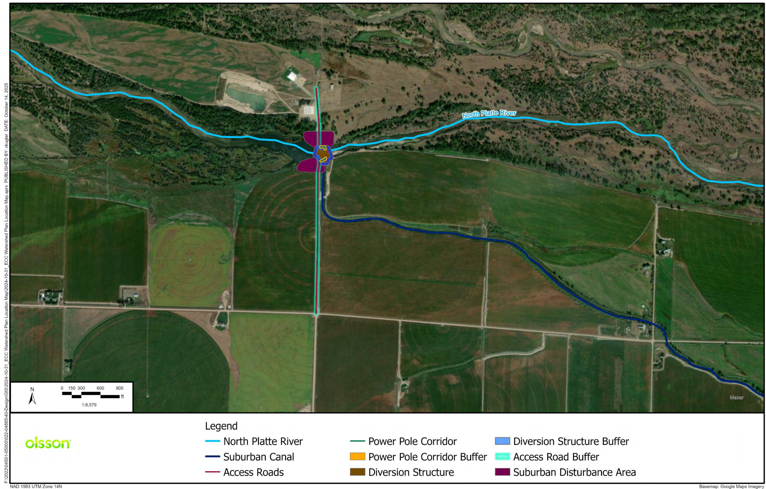
Figure 5: Suburban project detail map. Map of Suburban diversion with project details.
