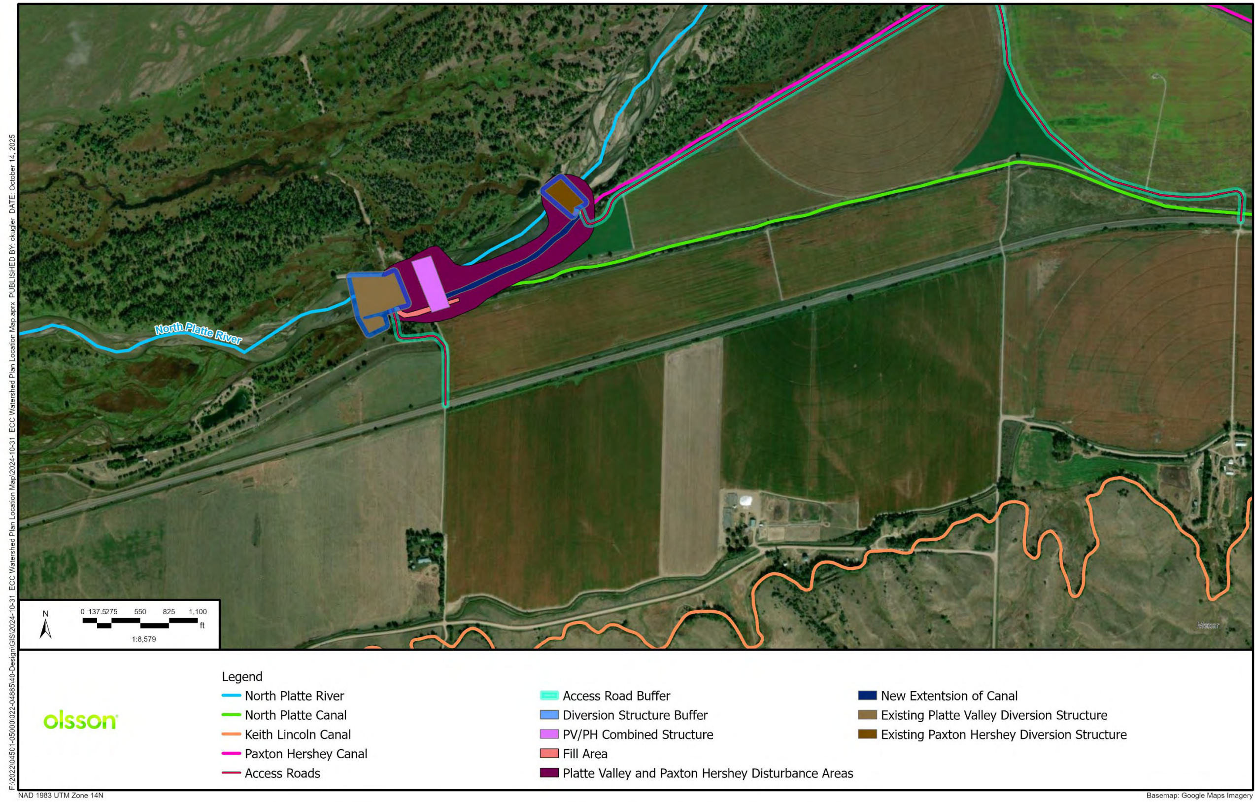
Figure 3: Platte Valley/Paxton-Hershey project detail map. Map of Platte Valley/Paxton-Hershey diversion with project details.
