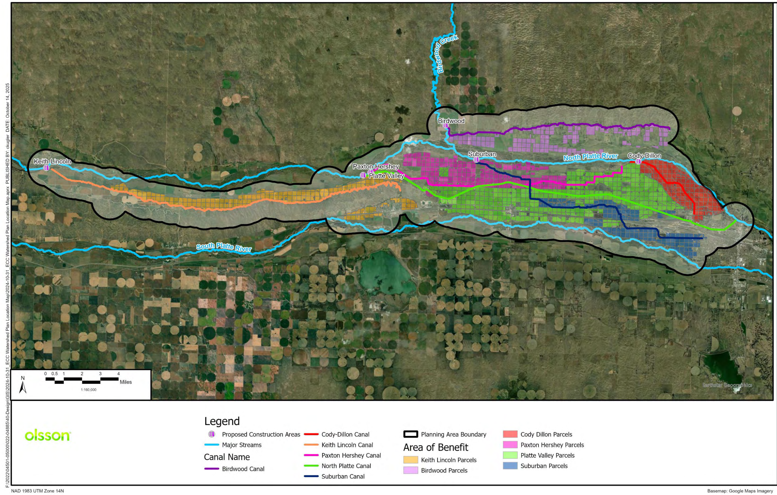
Figure 1: General project map with canals and area of benefit. Map of portions of Keith and Lincoln Counties showing the Planning Area with included canals and area of benefit.
