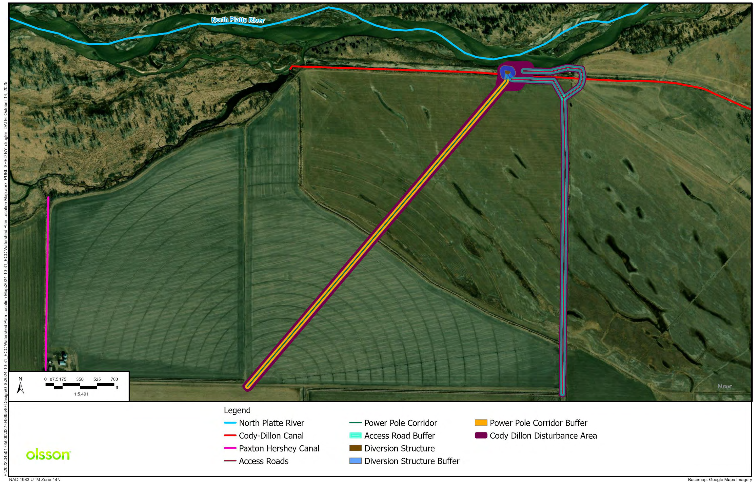
Figure 6: Cody-Dillon project detail map. Map of Cody-Dillon diversion with project details.
