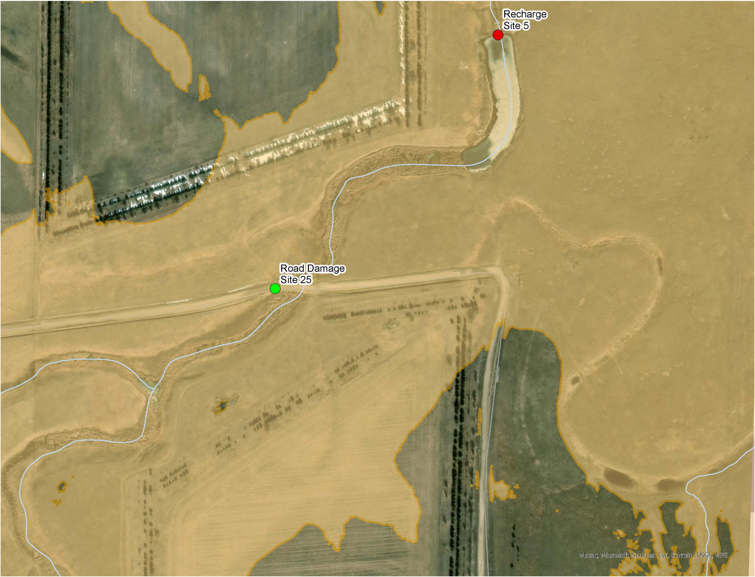
0.2-PERCENT AEP FLOODPLAIN EXISTING CONDITIONS BOX BUTTE CREEK WATERSHED PLAN & EA - ROADWAY SITE 25
