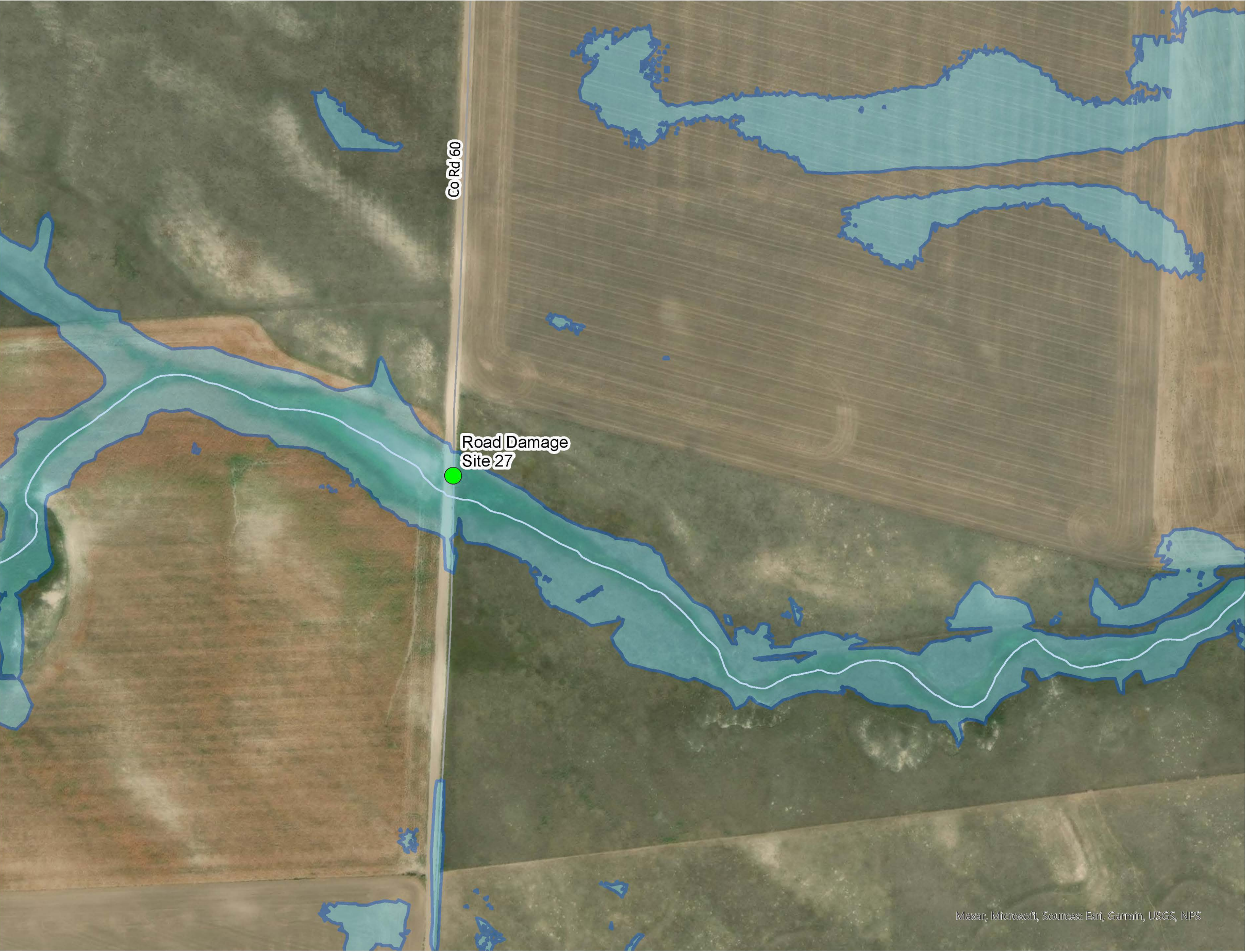
1-PERCENT AEP FLOODPLAIN EXISTING CONDITIONS BOX BUTTE CREEK WATERSHED PLAN & EA - ROADWAY SITE 27
