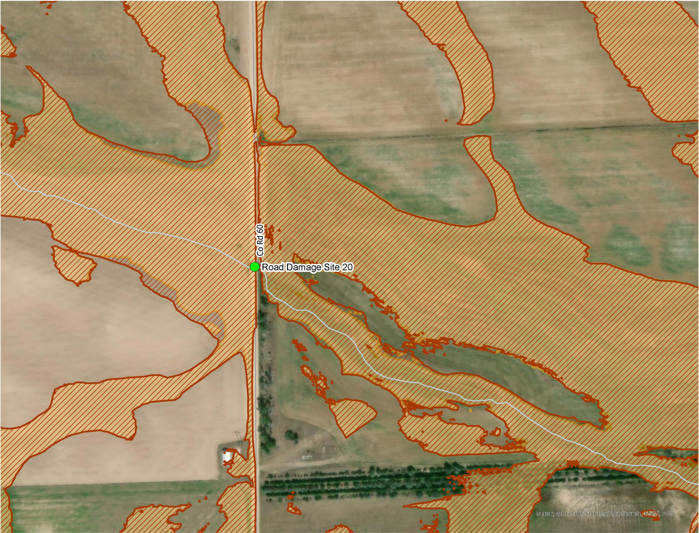
0.2-PERCENT AEP FLOODPLAIN WITH ROADWAY IMPROVEMENTS BOX BUTTE CREEK WATERSHED PLAN & EA - ROADWAY SITE 20
