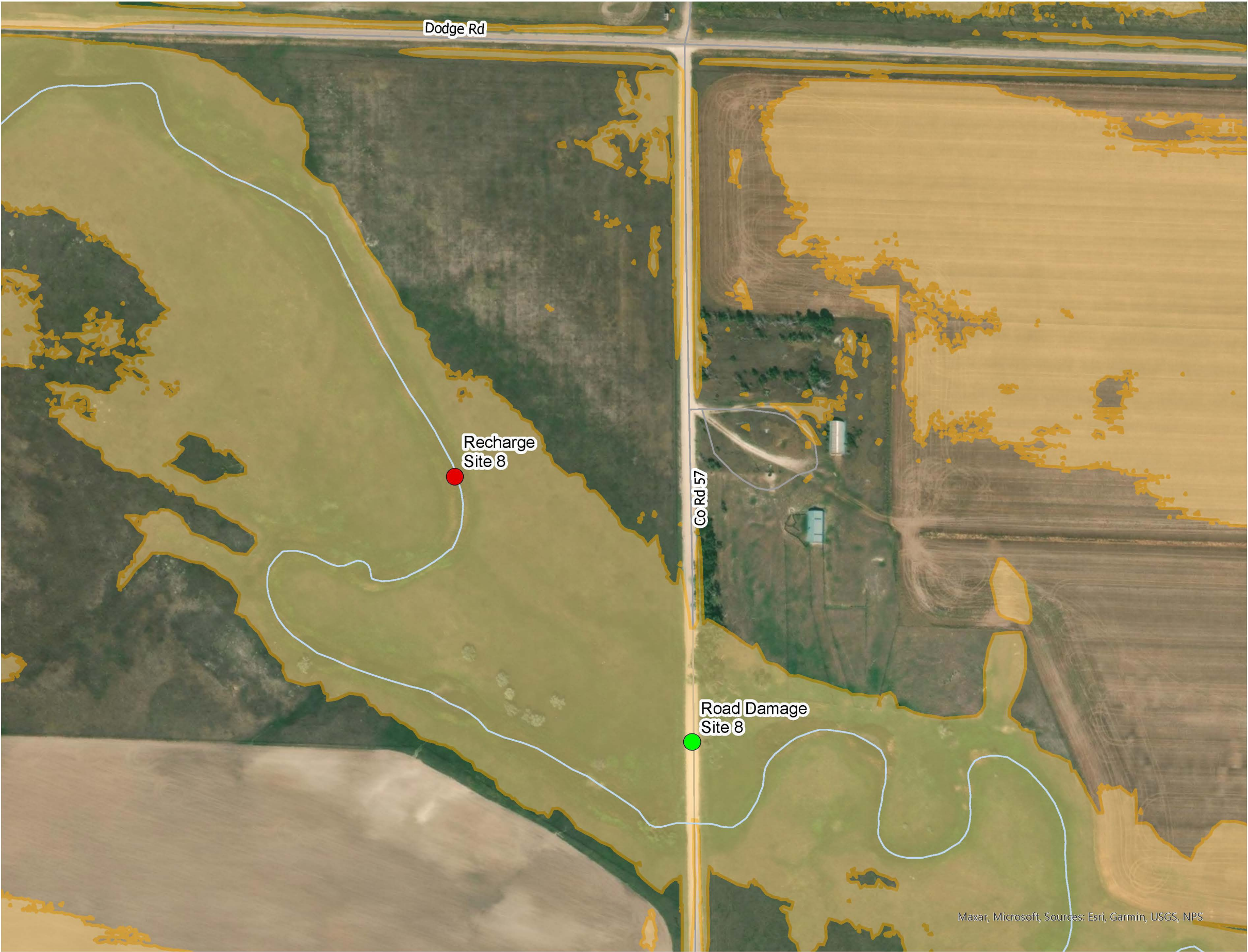
0.2-PERCENT AEP FLOODPLAIN EXISTING CONDITIONS BOX BUTTE CREEK WATERSHED PLAN & EA - SITE 8 FIGURE 5-5 G-3
