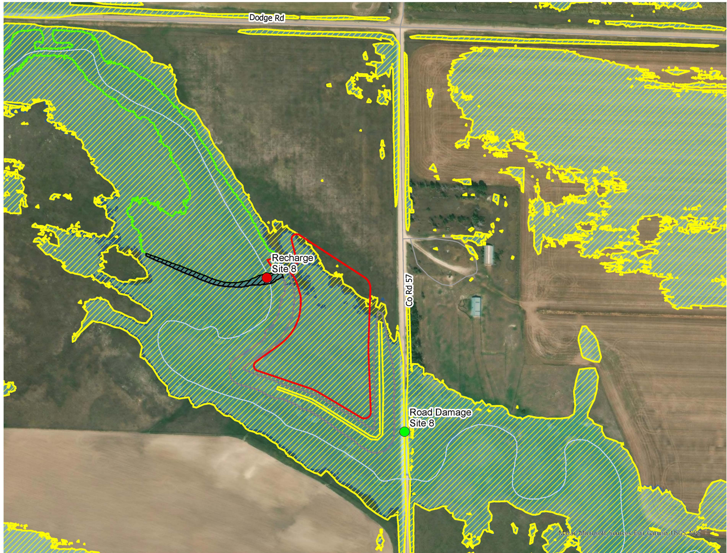
1-PERCENT AEP FLOODPLAIN WITH RECHARGE PROJECT BOX BUTTE CREEK WATERSHED PLAN & EA - RECHARGE SITE 8
