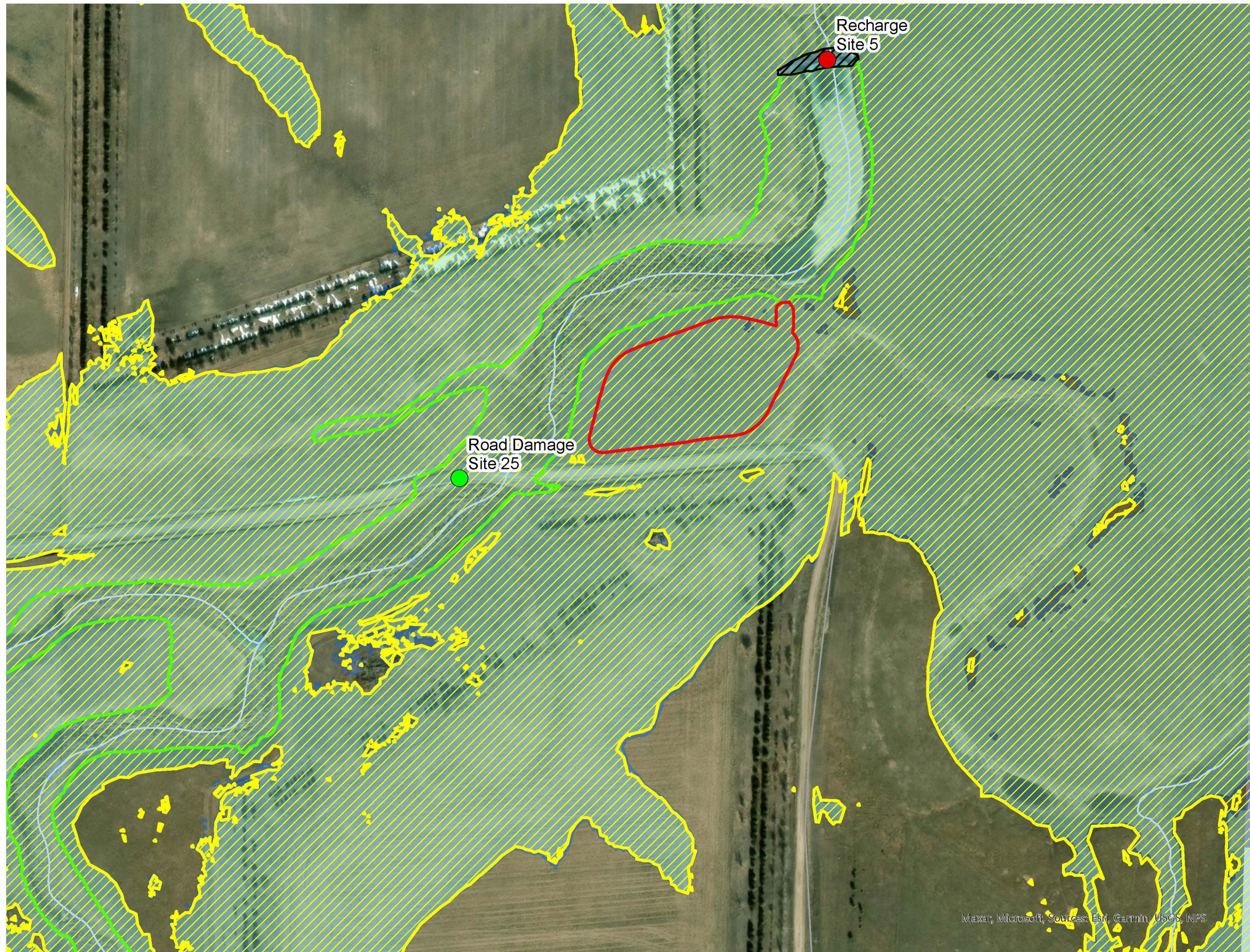
1-PERCENT AEP FLOODPLAIN WITH ROADWAY IMPROVEMENTS BOX BUTTE CREEK WATERSHED PLAN & EA - ROADWAY SITE 25
