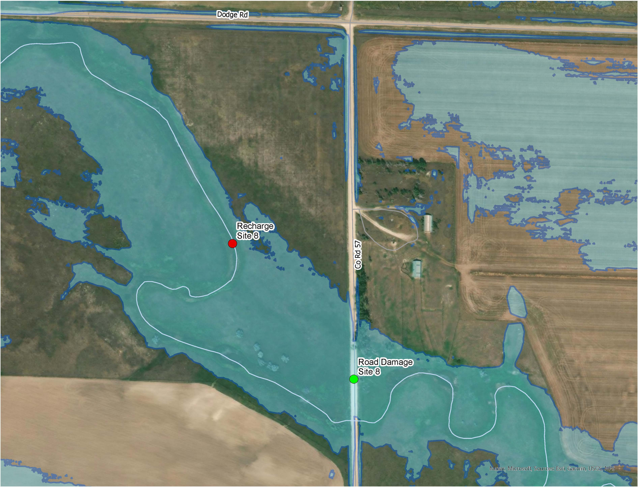
1-PERCENT AEP FLOODPLAIN EXISTING CONDITIONS BOX BUTTE CREEK WATERSHED PLAN & EA - RECHARGE SITE 8
