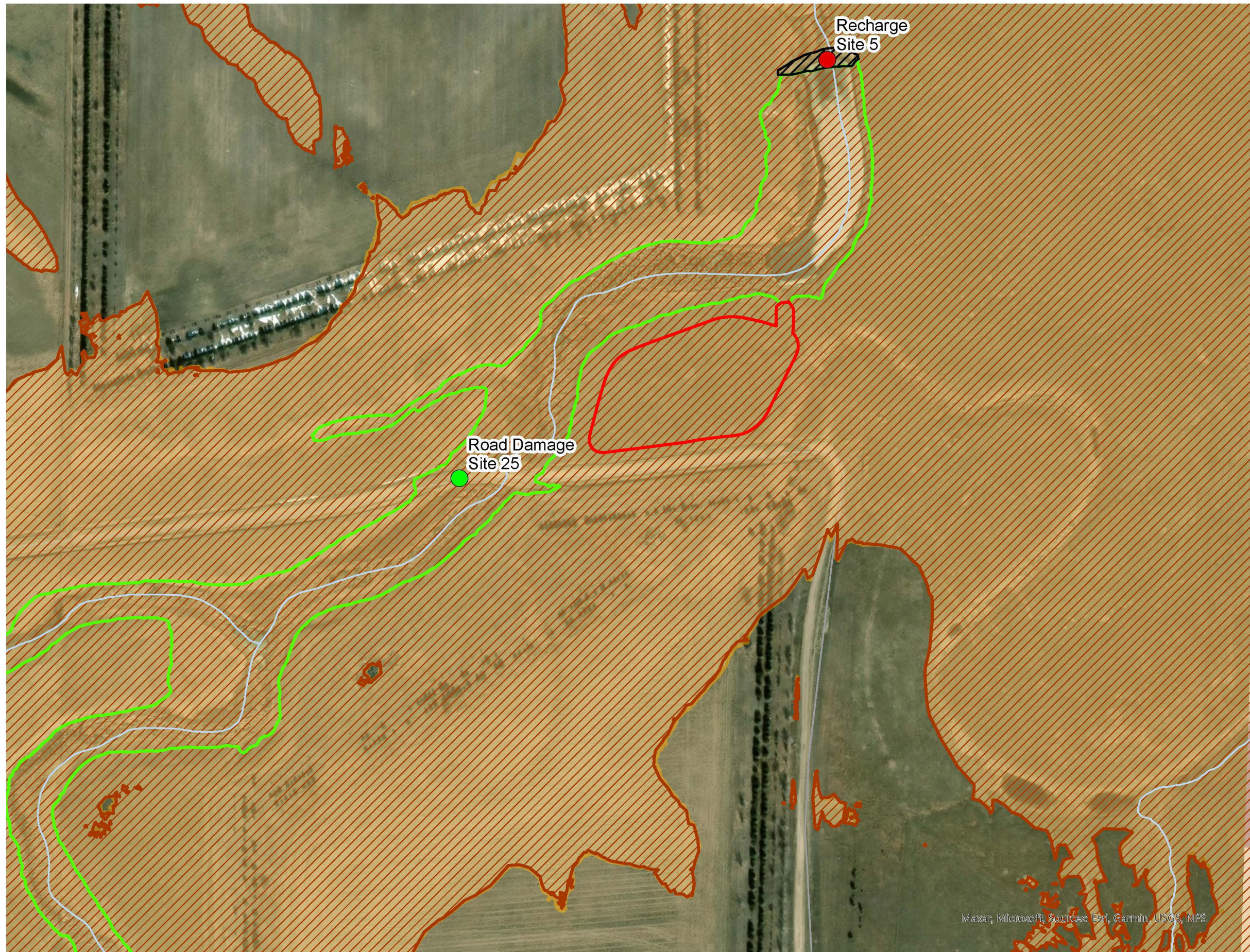
0.2-PERCENT AEP FLOODPLAIN WITH ROADWAY IMPROVEMENTS BOX BUTTE CREEK WATERSHED PLAN & EA - ROADWAY SITE 25
