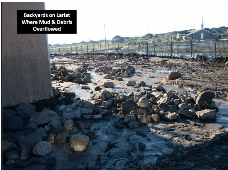
Figure E-6 Typical sediment composition in residential area
