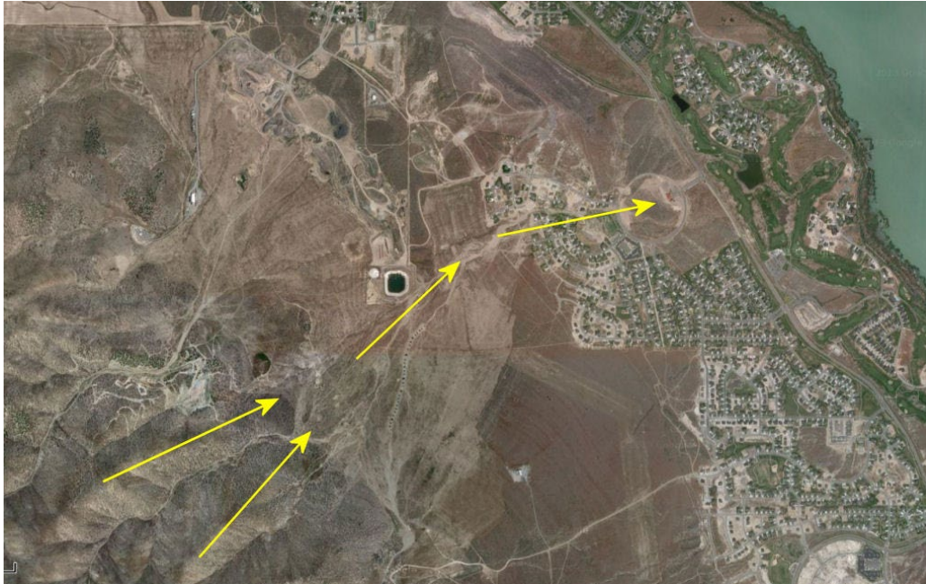
Figure E-4 Burned watershed flow direction into Saratoga Springs from September 2012 event
