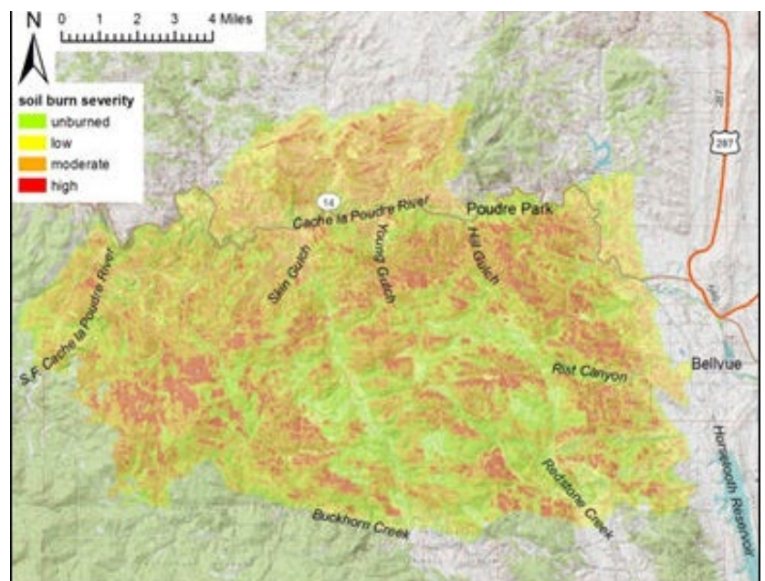
Figure A–2 Aerial extent and soil burn severity of the High Park fire, based on a BARC image
