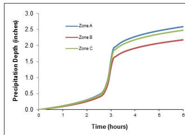
Figure C-5 Twenty-five-year cumulative rainfall distributions used in modeling
