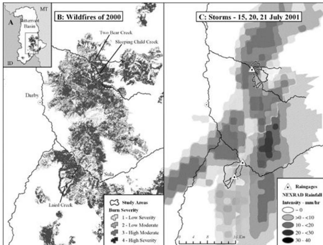
Figure B-11 Burn severity and rain gage data for storm event 1-year post-fire
