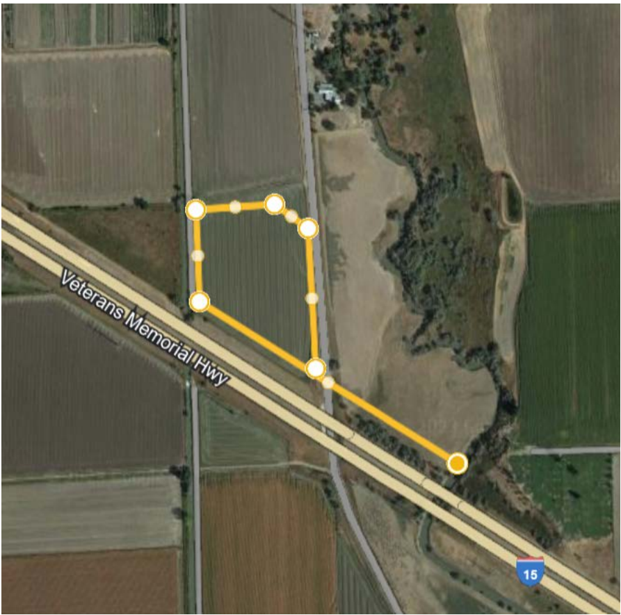
100 East – I15 Flood Control Piping to Malad River
