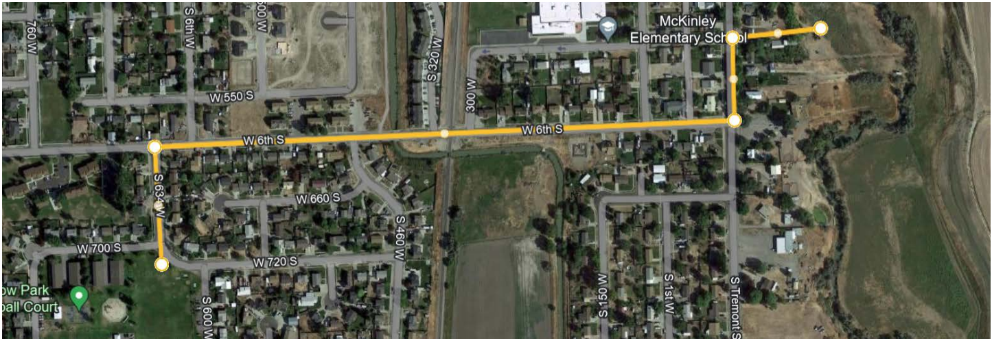
600 South Flood Control Piping to Malad River
