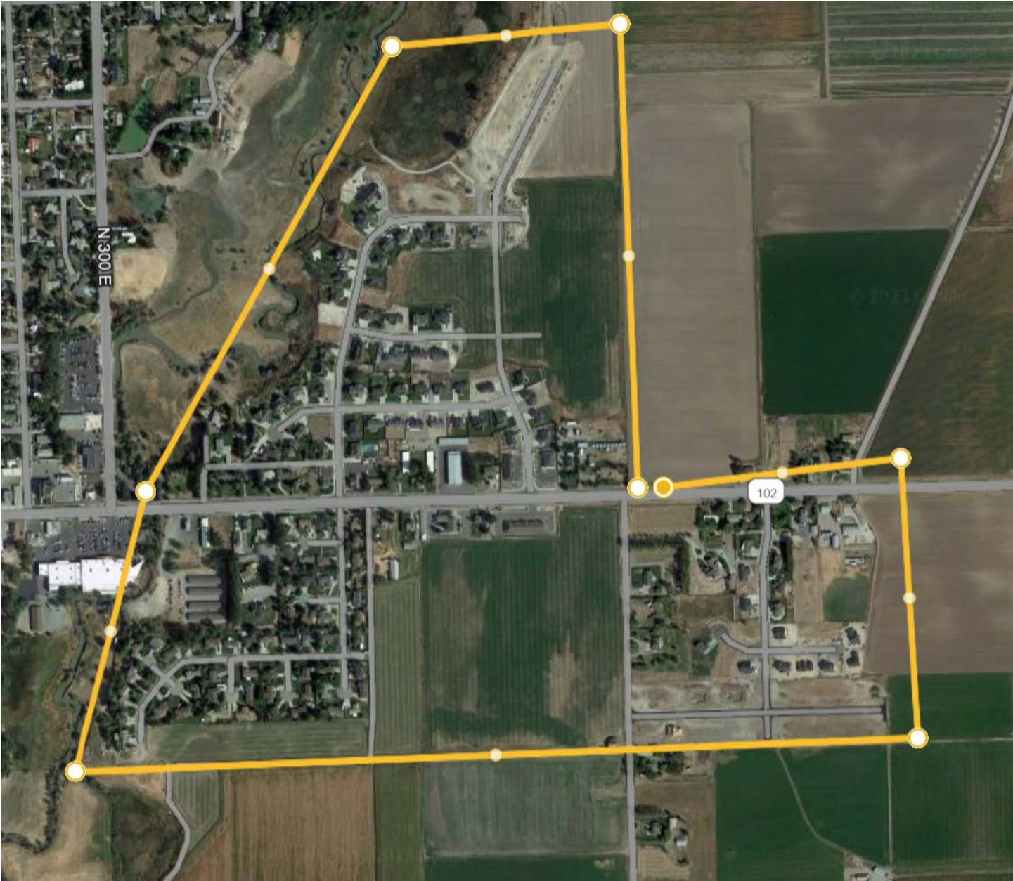
Service Area 9 Secondary Distribution Piping
