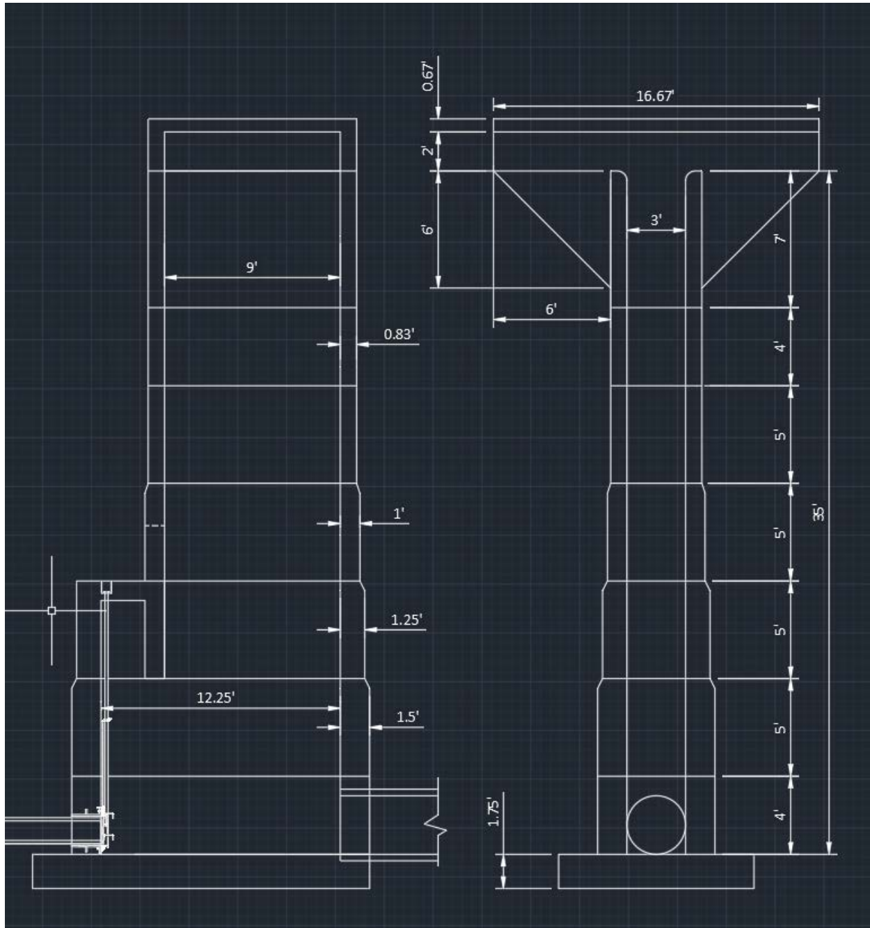
Elevation Views
