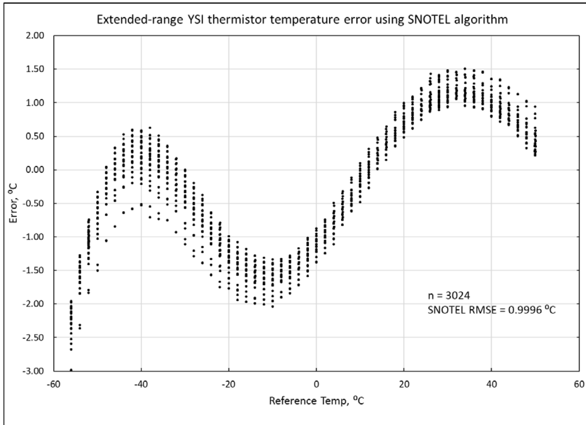
Figure 2. Difference between temperature calculated using the SNOTEL algorithm and the reference temperature.
