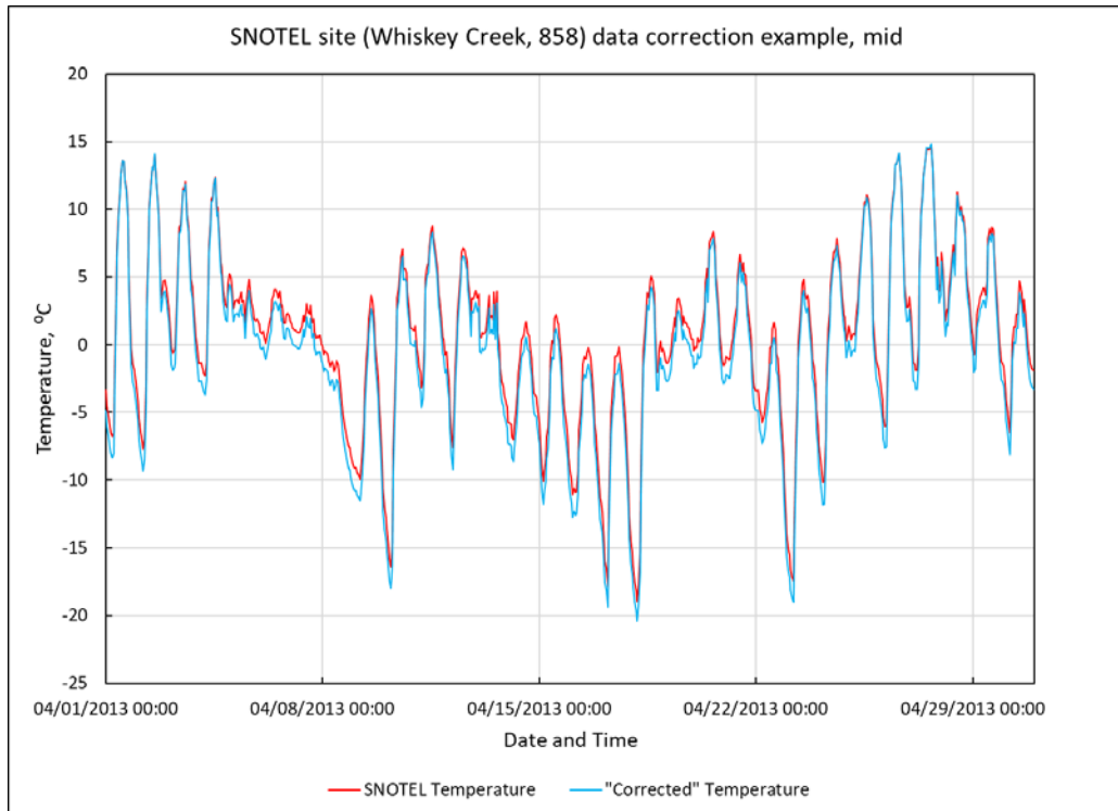
Figure 8. Transformation of historic temperature data from the Whiskey Creek SNOTEL site, mid-range temperature values.
