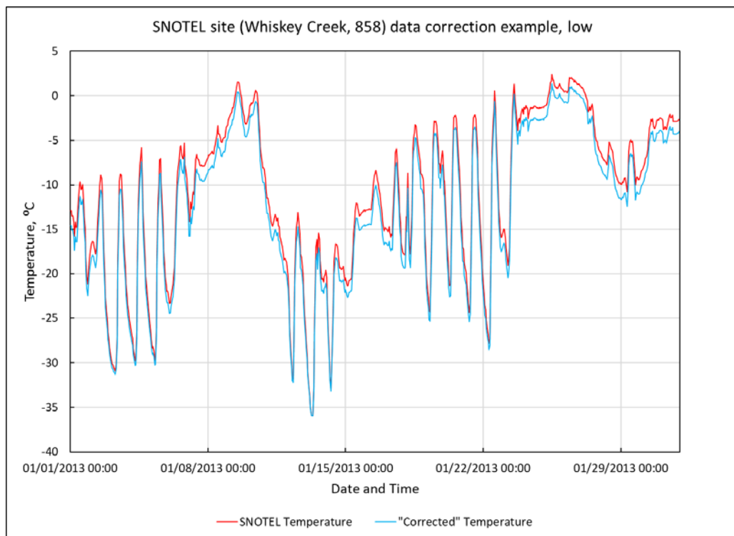
Figure 7. Transformation of historic temperature data from the Whiskey Creek SNOTEL site, low-range temperature values.
