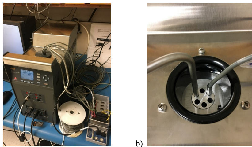
Figure 1. a) Temperature test setup: dry-well calibrator, platinum resistance thermometer, data acquisition hardware, thermistors in test. b) Close-up of dry-well calibrator test chamber and insert.
