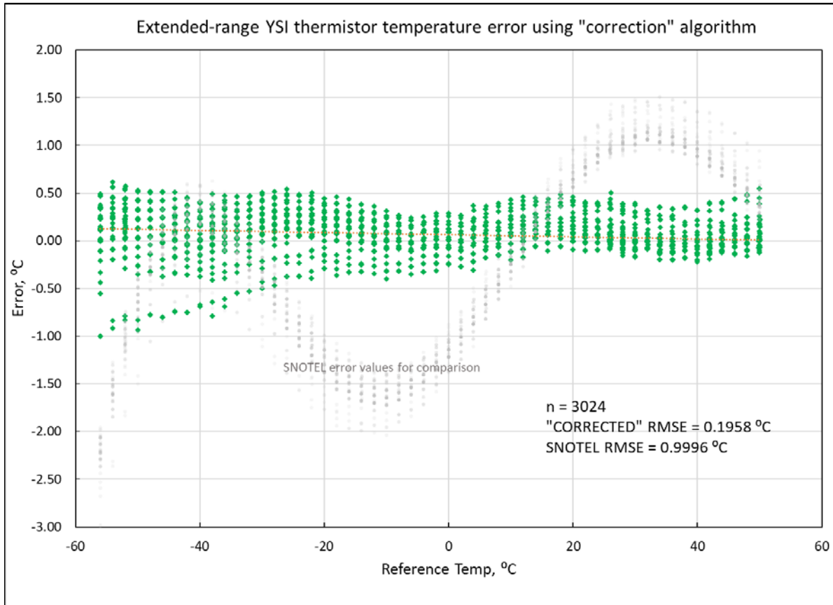
Figure 5. Difference between temperature calculated using the algorithm developed in this study and the reference temperature.
