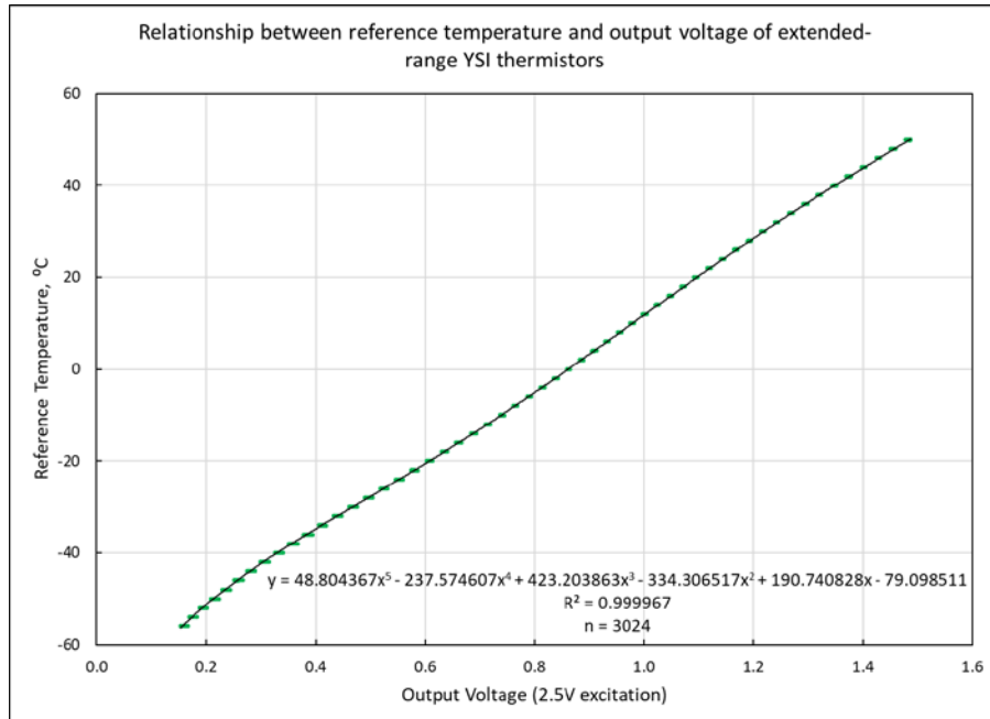
Figure 3. Relationship between the reference temperature and the output voltage of the extended-range YSI thermistors.
