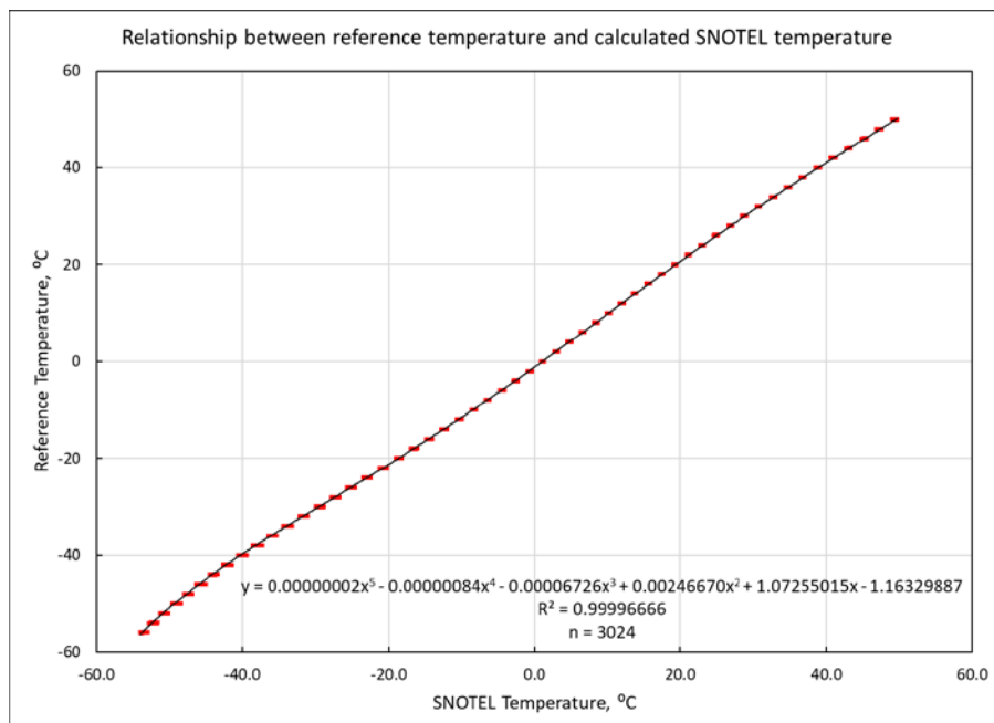
Figure 4. Relationship between the reference temperature and temperature calculated from thermistor output voltage using the SNOTEL algorithm.
