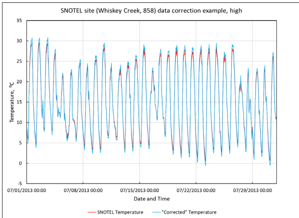
Figure 9. Transformation of historic temperature data from the Whiskey Creek SNOTEL site, high-range temperature values.
