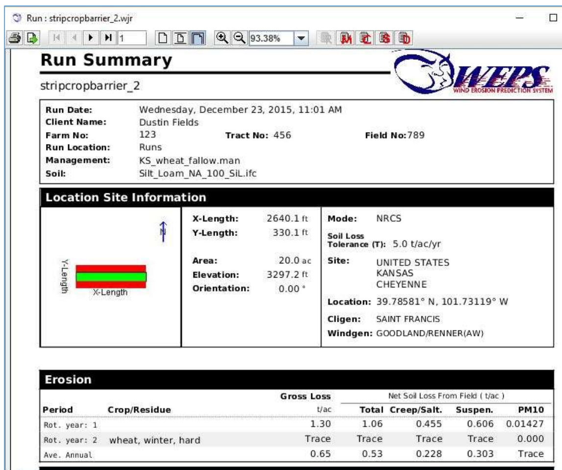
Figure 6-28 Run Summary report for the strip-cropped field with barriers.
