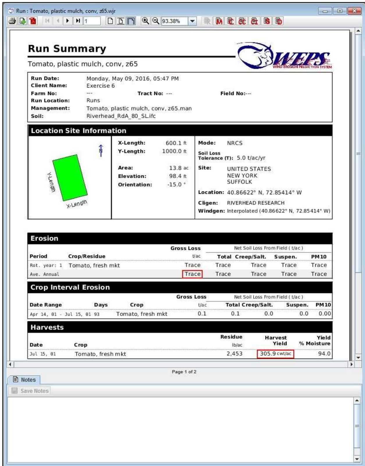
Figure 4-77 Run Summary after adding the plastic mulch.
