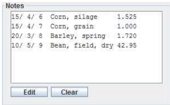
Figure 2-10 Notes panel for documenting pending WEPS simulation run information.
