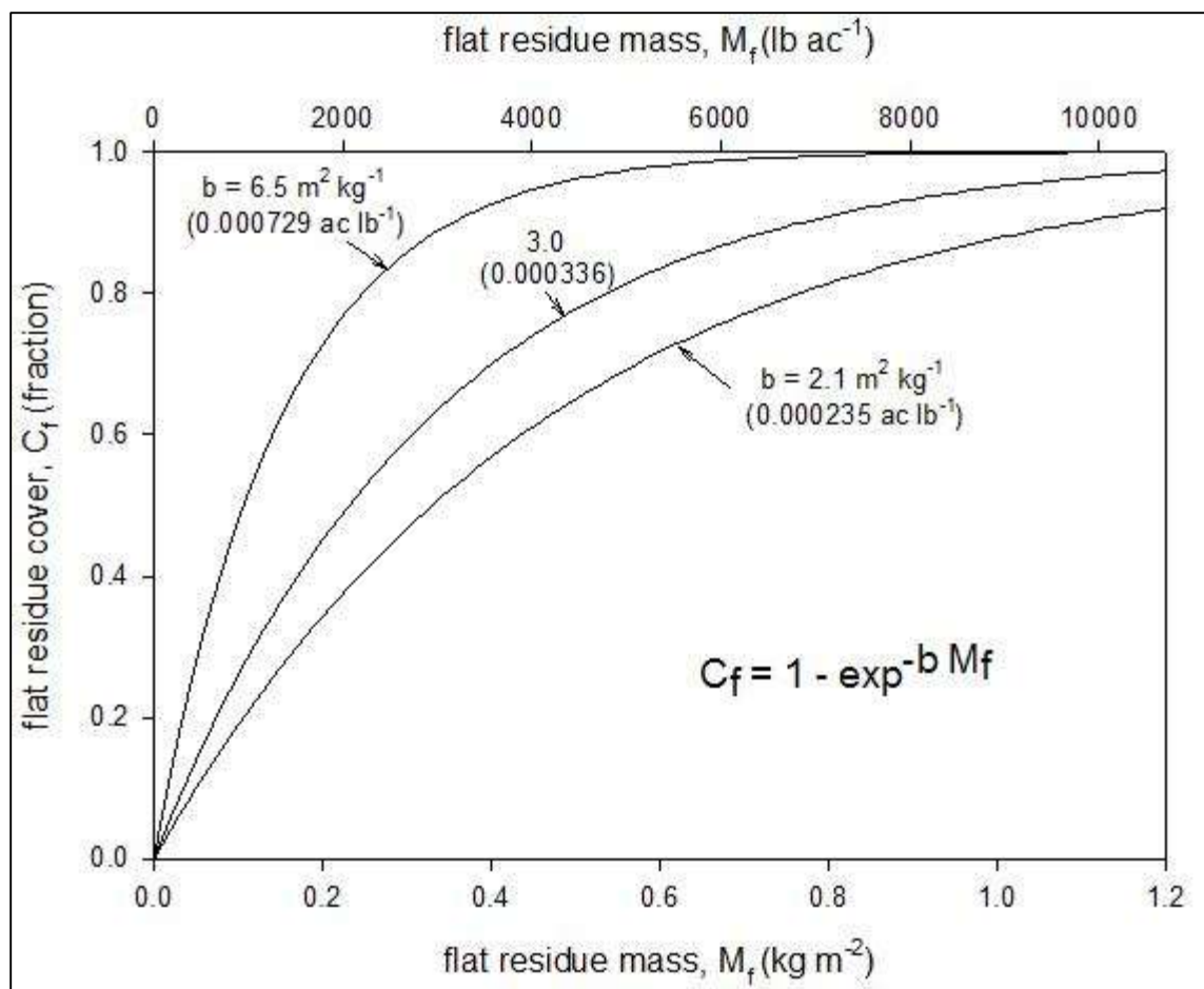
Figure 6-43 Relationship between flat residue mass and the cover provided by this flat residue.
