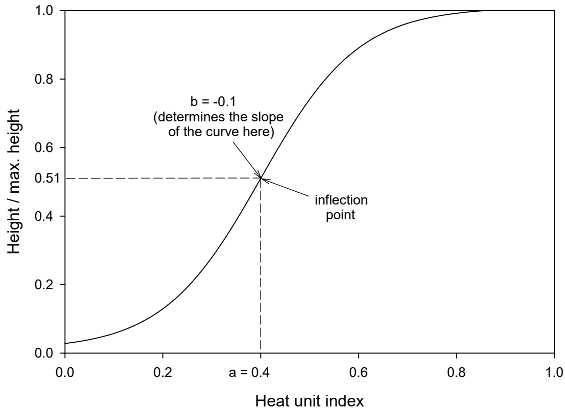
Figure 6-38 Crop height development function as it would be without any stresses. In this example, a = 0.4 and b = -0.1 . The height ratio at the inflection point = 0.51.
