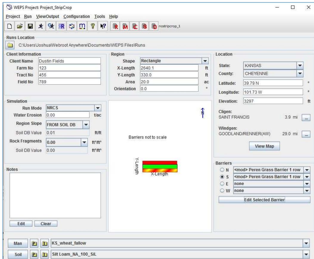
Figure 6-27 Main screen showing the setup for a field strip-cropped with grass barriers.
