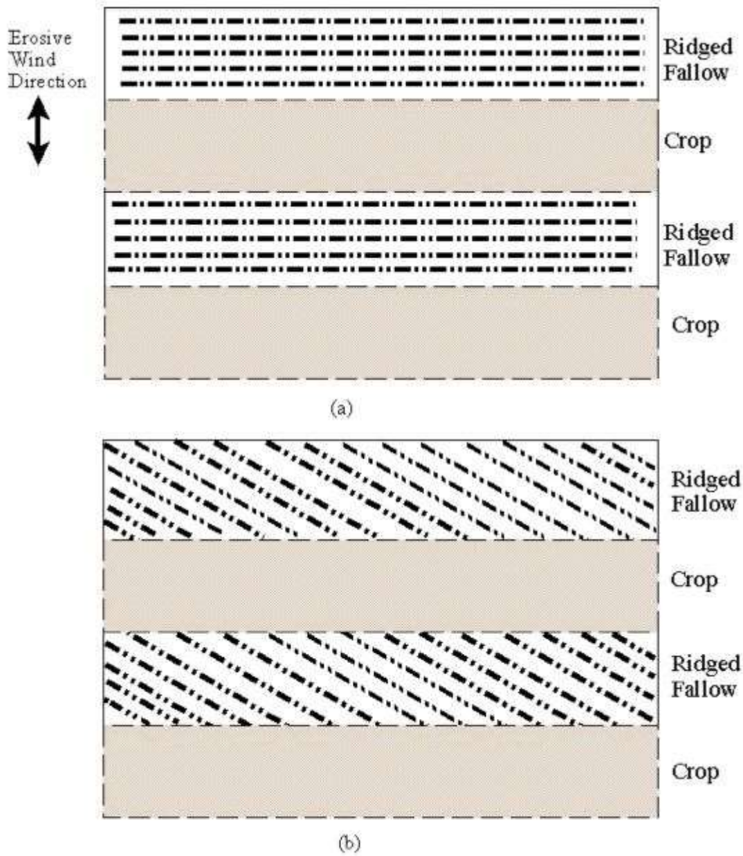
Figure 6-16 Designs using (a) parallel tillage ridges and (b) angled tillage ridges.
