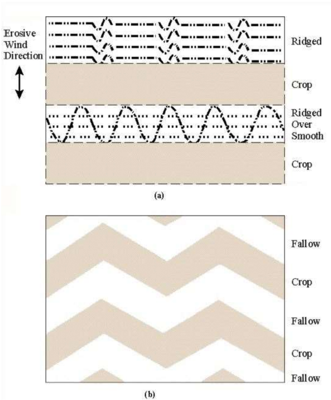
Figure 6-17 Erosion control designs using (a) variations of curved ridges and (b) curved strips.
