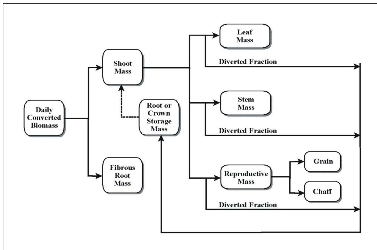
Figure 6-34 Schematic of biomass partitioning in WEPS. Biomass is converted from solar radiation and partitioned to ‘fibrous root’ and ‘shoot’ parts. The shoot mass is partitioned into leaf, stem, and reproductive masses, with some fraction of these masses diverted into a storage pool for crop regrowth. Finally, the reproductive mass is partitioned into grain and chaff parts.
