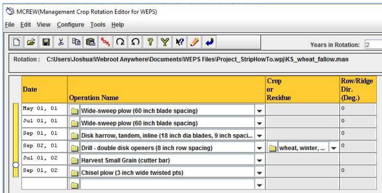
Figure 6-20 Management Crop Rotation Editor for a conventional wheat fallow rotation.
