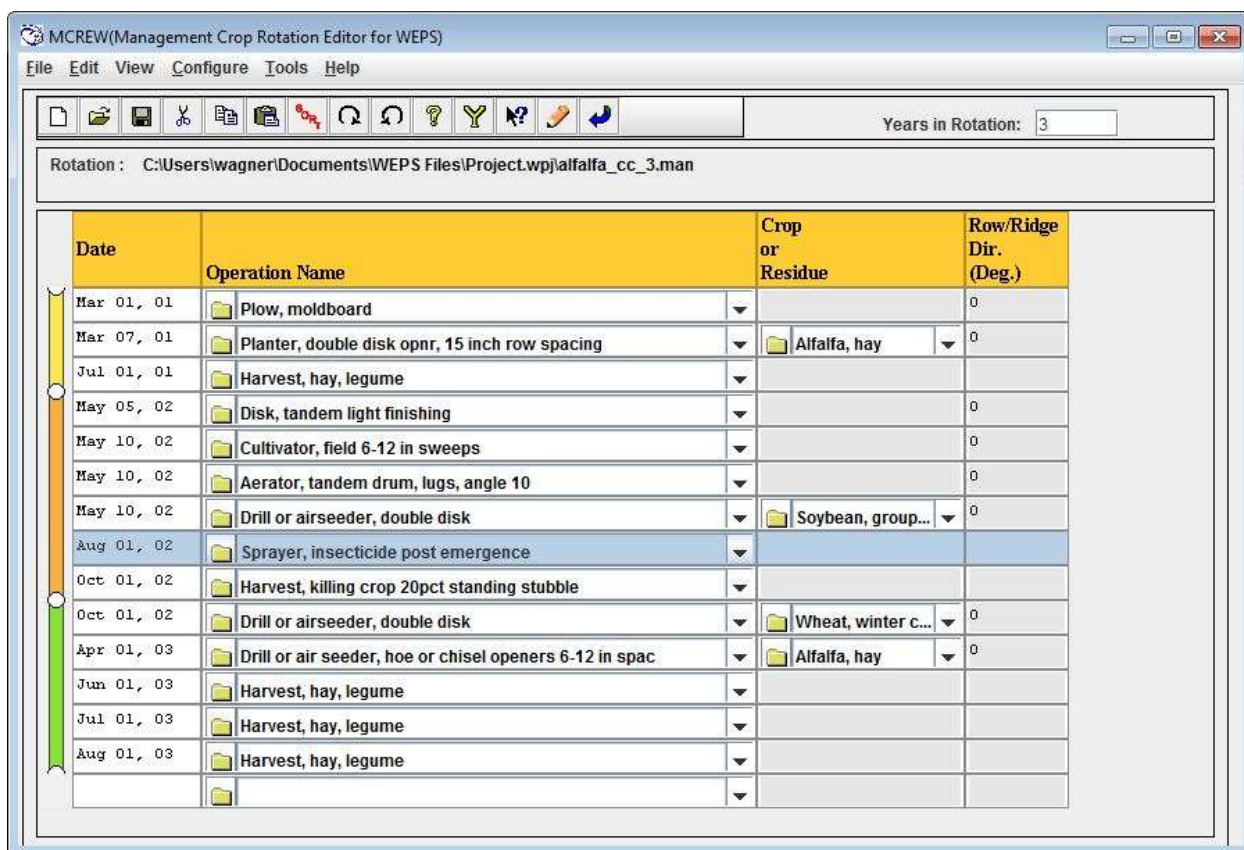
Figure 2-20 Management/Crop Rotation Editor for WEPS (MCREW) window.
