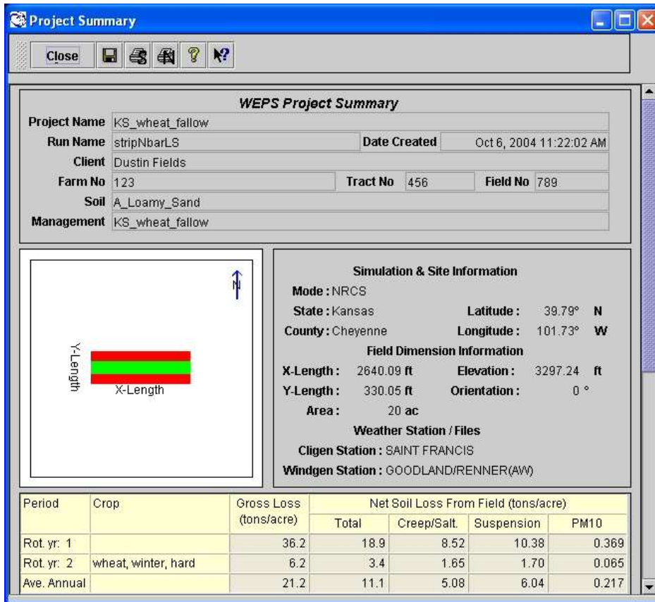
Figure 6-32 Run Summary for the strip-cropped scenario of loamy sand with barriers.
