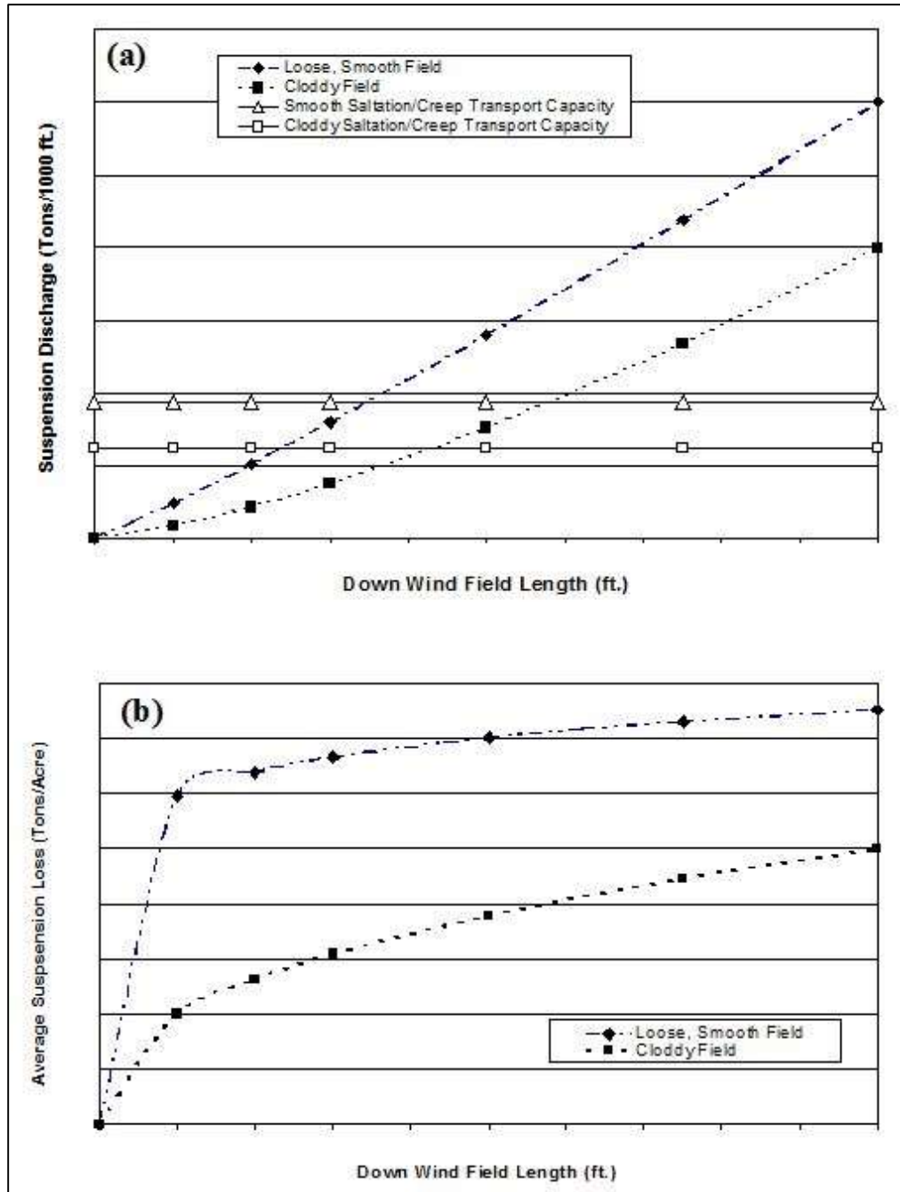
Figure 6-12 Downwind (a) discharge per 100 ft. of border width and (b) average soil loss of suspended soil.
