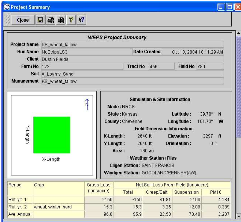
Figure 6-30 Run Summary for the non-stripped scenario with a loamy sand soil.
