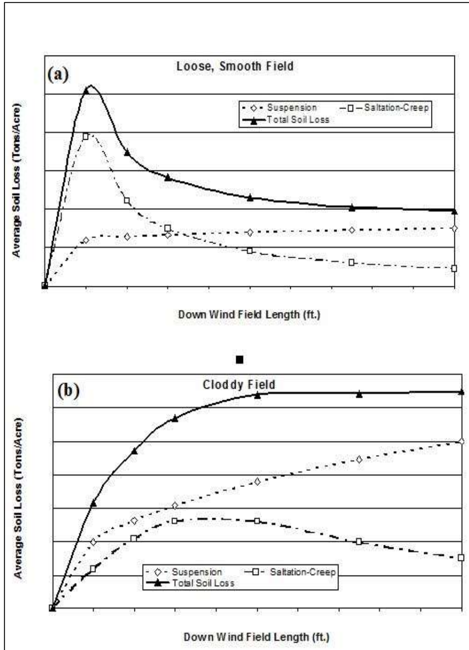
Figure 6-13 Comparison of average soil loss at various downwind distances on (a) a smooth, loose field and (b) a cloddy field.
