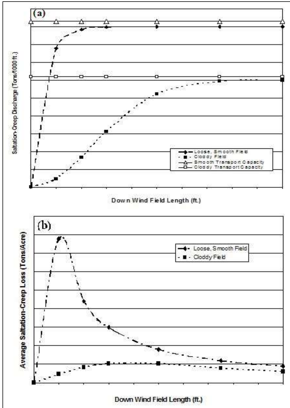
Figure 6-11 Comparison of (a) downwind discharge per 100 ft. of border width and (b) average soil loss for saltation-creep.
