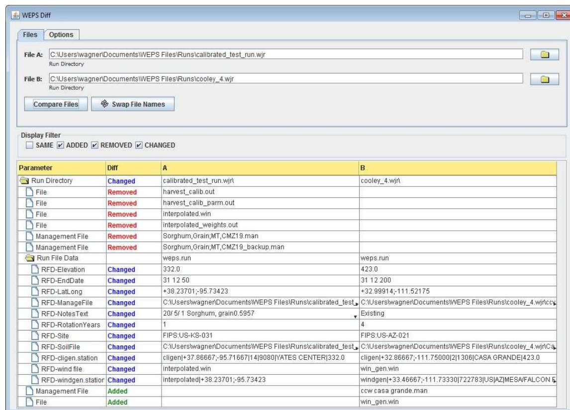
Figure 2-63 WEPS Differencing Window.
