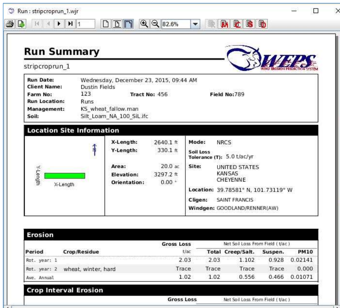
Figure 6-24 Run Summary report for the strip-cropped scenario.
