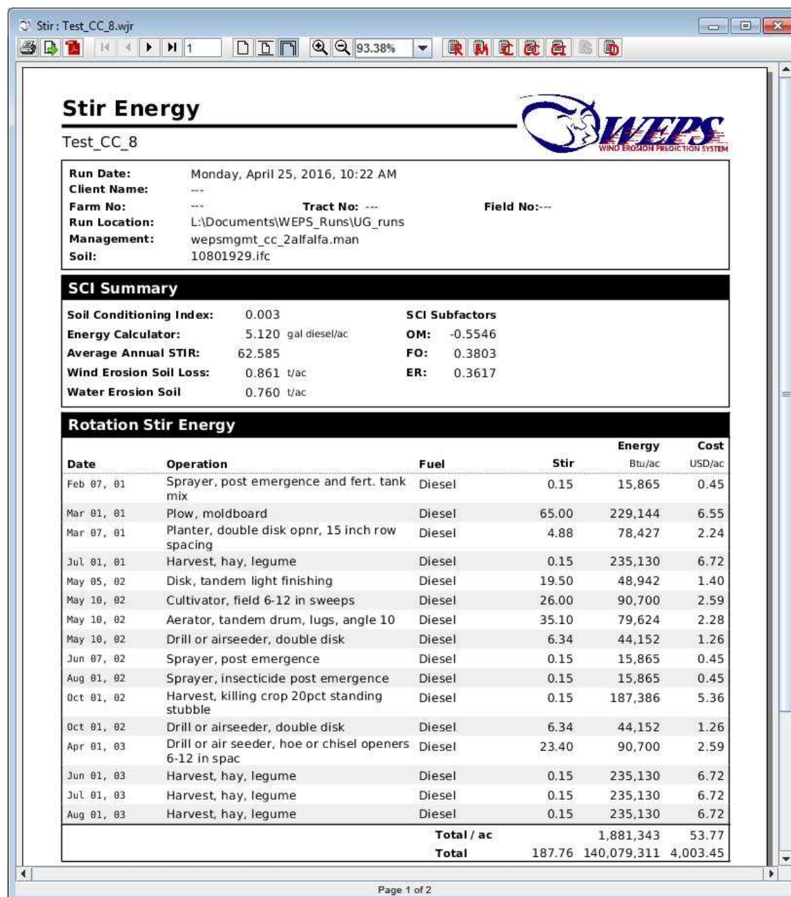
Figure 2-48 WEPS STIR Energy Report displaying the “SCI Summary” and “Rotation STIR Energy” sections.
