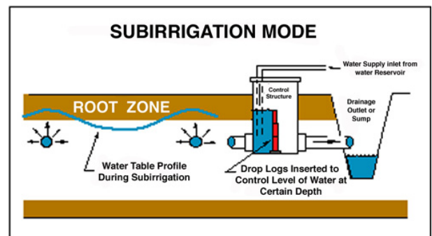
Subirrigation System
