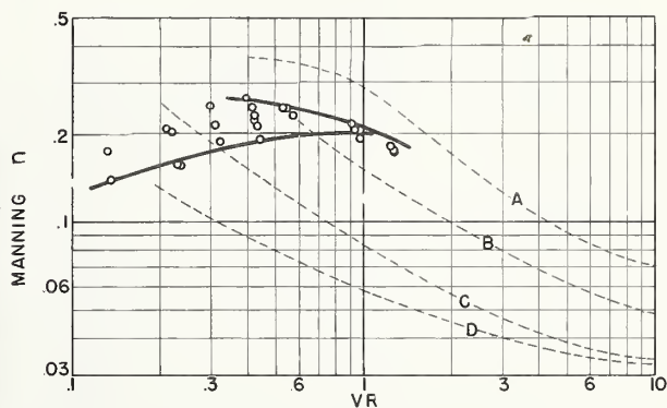
FIGURE 17.—Relation of Manning n to product of velocity and hydraulic radius ( VR ) for flow tests on channel FC 29, experiment 5.
