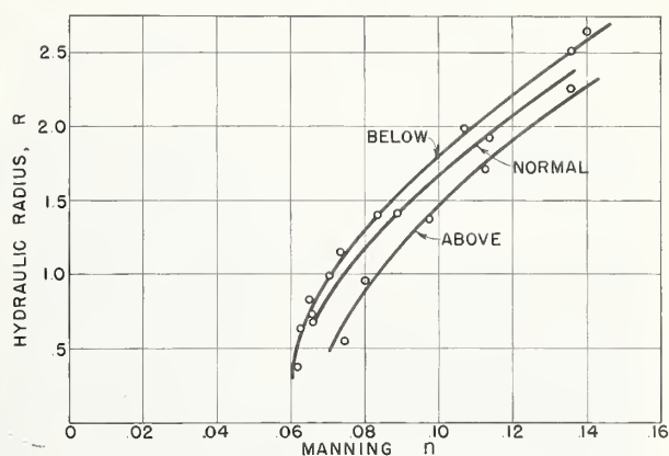
FIGURE 35.—Relation of Manning n to hydraulic radius ( R ) for flow tests on channel FC 30, experiment 4. (The three curves result from three flow-depth conditions—below normal, normal, and above normal.)
