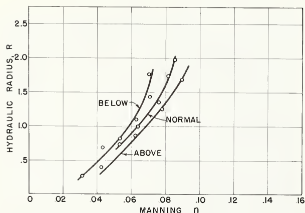
FIGURE 38.—Relation of Manning n to hydraulic radius ( R ) for flow tests on channel FC 29, experiment 4. (The three curves result from three flow-depth conditions—below normal, normal, and above normal.)
