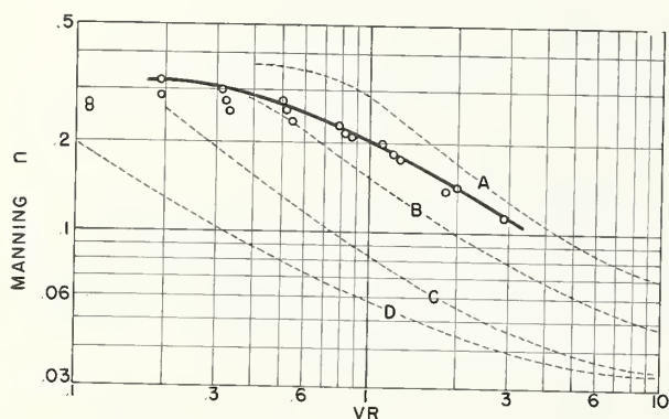
FIGURE 44.—Relation of Manning n to product of velocity and hydraulic radius ( VR ) for flow tests on channel FC 30, experiment 6.
