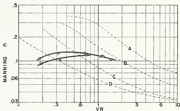
FIGURE 11.—Relation of Manning n to product of velocity and hydraulic radius ( VR ) for flow tests on channel FC 29, experiment 3.
