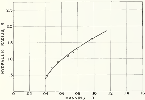
FIGURE 29.—Relation of Manning n to hydraulic radius ( R ) for flow tests on channel FC 29, experiment 2.
