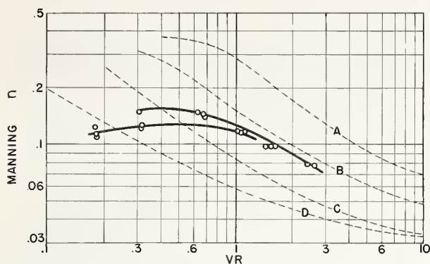
FIGURE 14.—Relation of Manning n to product of velocity and hydraulic radius ( VR ) for flow tests on channel FC 30, experiment 3.
