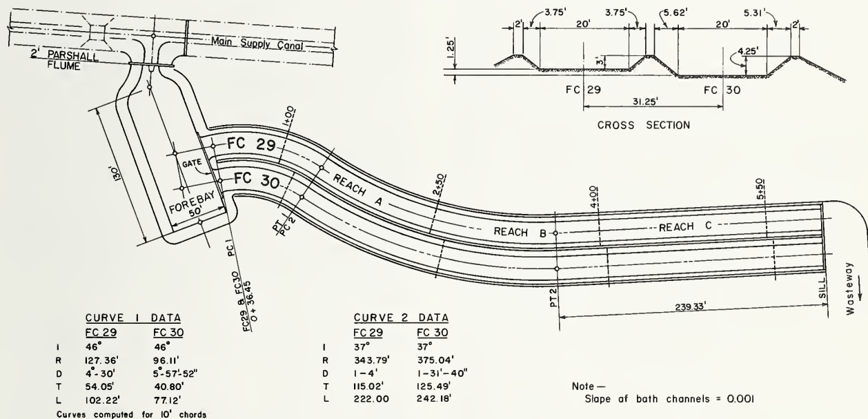
FIGURE 1.—Plan of test channels and forebay.
