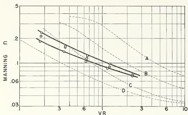
FIGURE 48.—Relation of Manning n to product of velocity and hydraulic radius ( VR ) for flow tests on channel FC 29, experiment 8.
