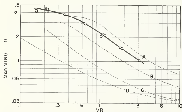
FIGURE 20.—Relation of Manning n to product of velocity and hydraulic radius ( VR ) for flow tests on channel FC 30, experiment 5.
