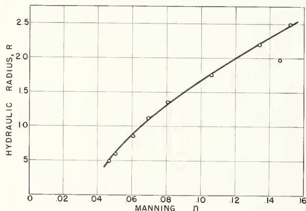
FIGURE 32.—Relation of Manning n to hydraulic radius ( R ) for flow tests on channel FC 30, experiment 2.
