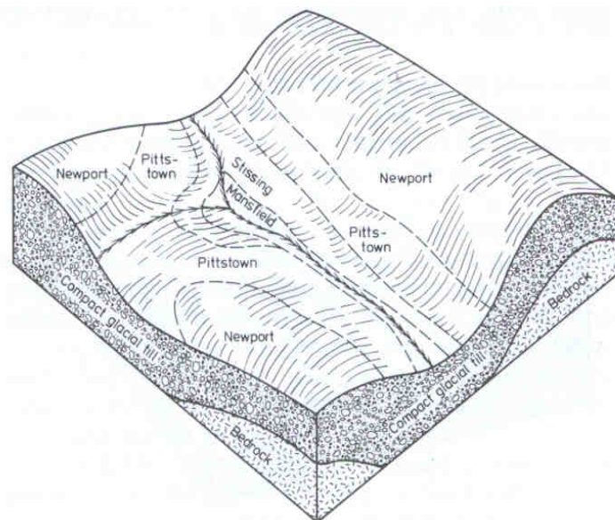
Figure 14. Block diagram illustrating the soil-landscape relationships of the Newport catena which has developed in compacted glacial till.
