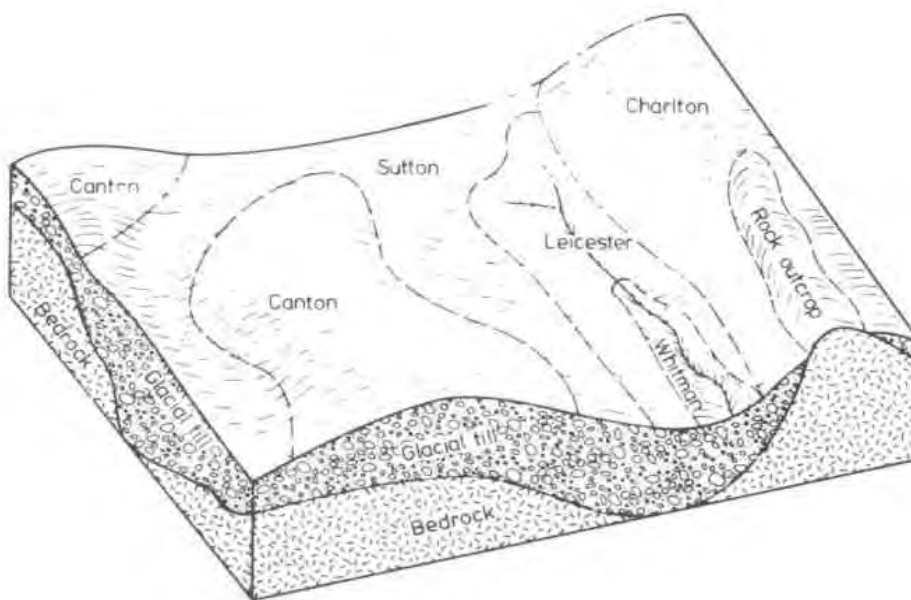
Figure 11. Block diagram illustrating the landscape relationships of soils developed in friable glacial till.
