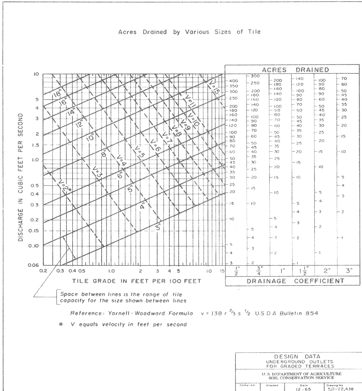
Exhibit 8-4 Tile design chart for underground outlets
