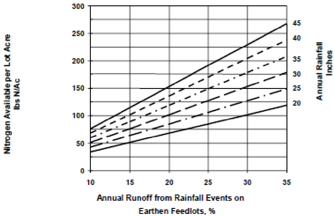
Figure 3. Annual N delivered to Wastewater Treatment Strips from earthen feedlots in pounds per acre. (From LPES Figure 22-10.)
