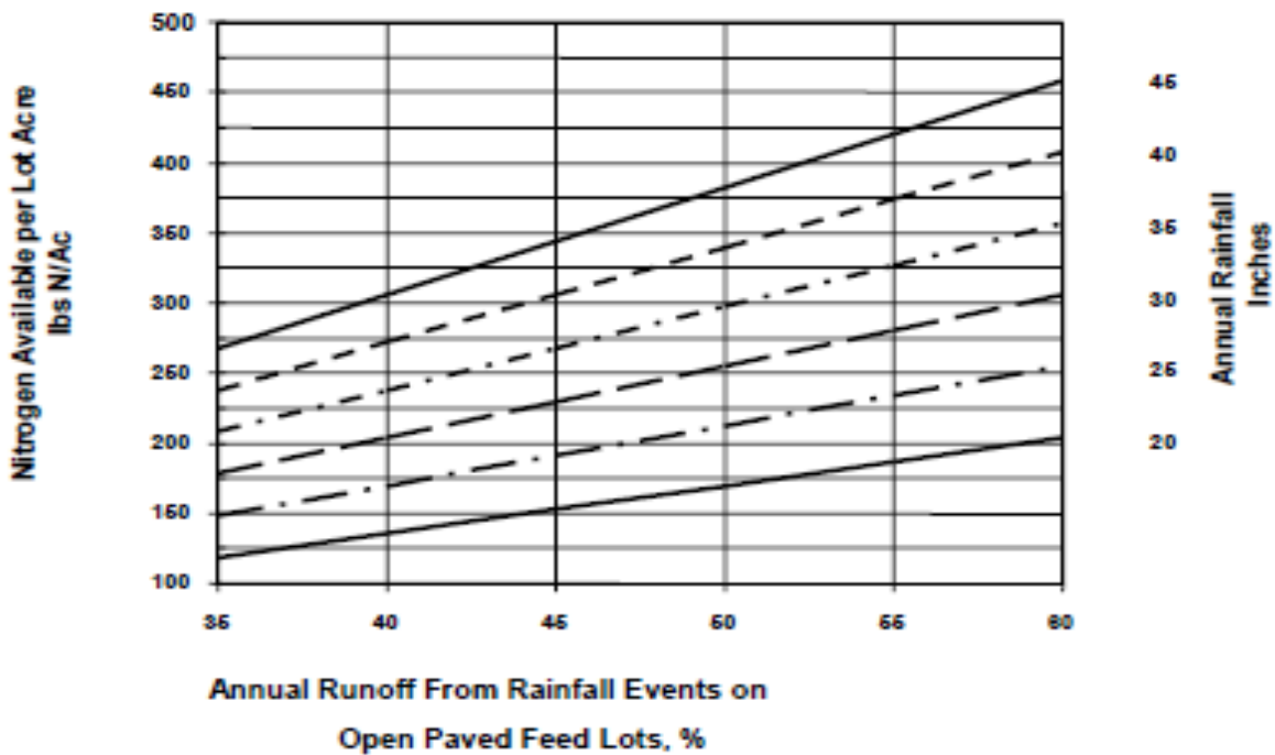
Figure 4. Annual N delivered to Wastewater Treatment Strips from paved feedlots in pounds per acre. (From LPES Figure 22-11.)
