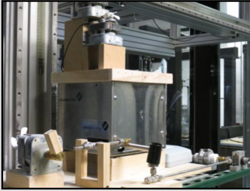
Apparatus used for dispensing, aerosolizing, and charge neutralizing calibration material into the aerosol wind tunnel
