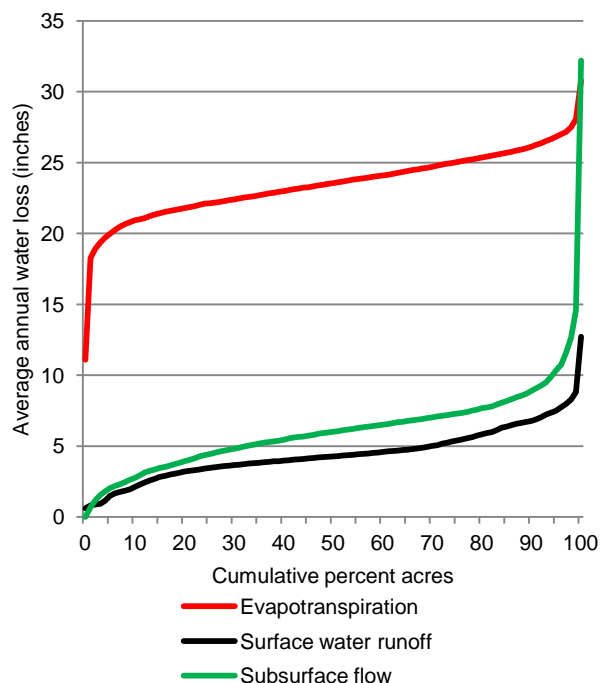
Figure 13. Estimates of average annual water lost through three loss pathways for cropped acres in the Upper Mississippi River Basin
