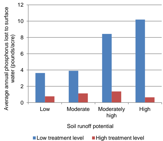
Figure 60. Trend in average annual phosphorus lost to surface water for increasing levels of soil runoff potential at two levels of conservation treatment, Upper Mississippi River Basin.
