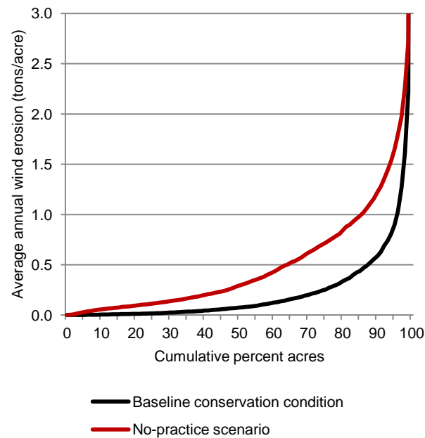
Figure 19. Estimates of average annual wind erosion for cropped acres in the Upper Mississippi River Basin
