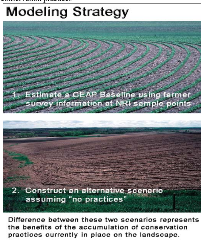
Figure 4. Modeling strategy used to assess effects of conservation practices
