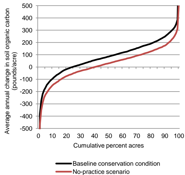
Figure 26. Estimates of average annual gain in soil organic carbon due to the use of conservation practices on cropped acres in the Upper Mississippi River Basin
