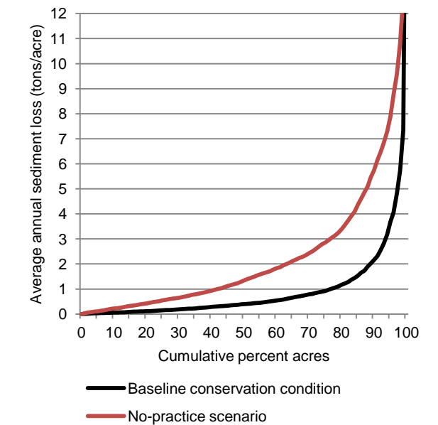
Figure 22. Estimates of average annual sediment loss for cropped acres in the Upper Mississippi River Basin
