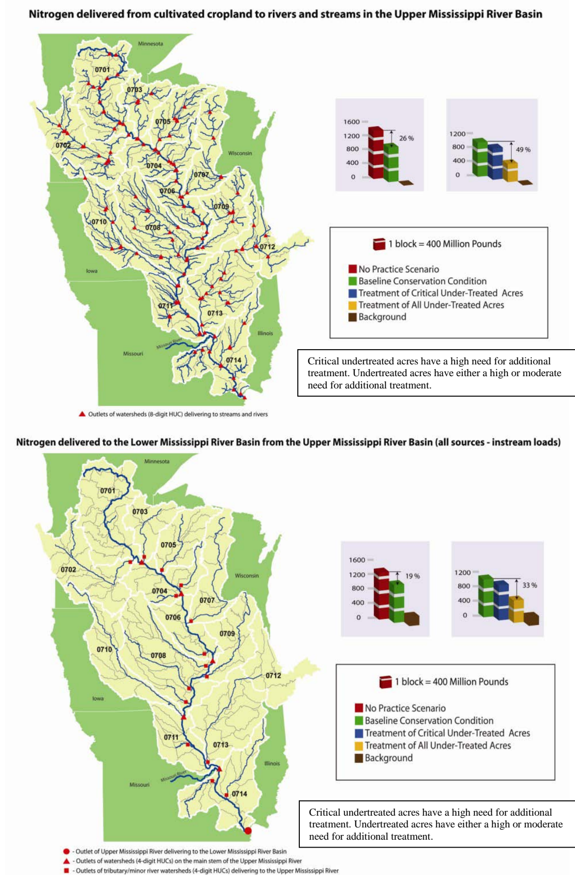
Figure 94. Summary of the effects of conservation practices on total nitrogen loads in the Upper Mississippi River Basin
