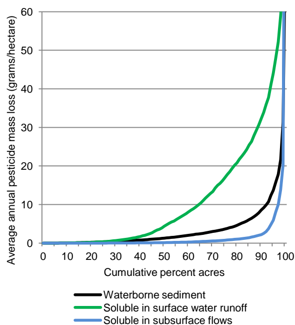
Figure 44. Estimates of average annual pesticide loss (mass loss of all pesticides combined) for three loss pathways, Upper Mississippi River Basin, baseline conservation condition
