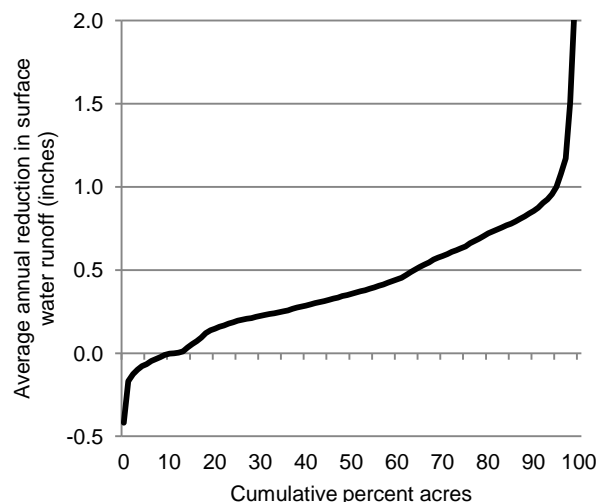
Figure 17. Estimates of average annual reduction in surface water runoff due to conversion to long-term conserving cover in the Upper Mississippi River Basin
