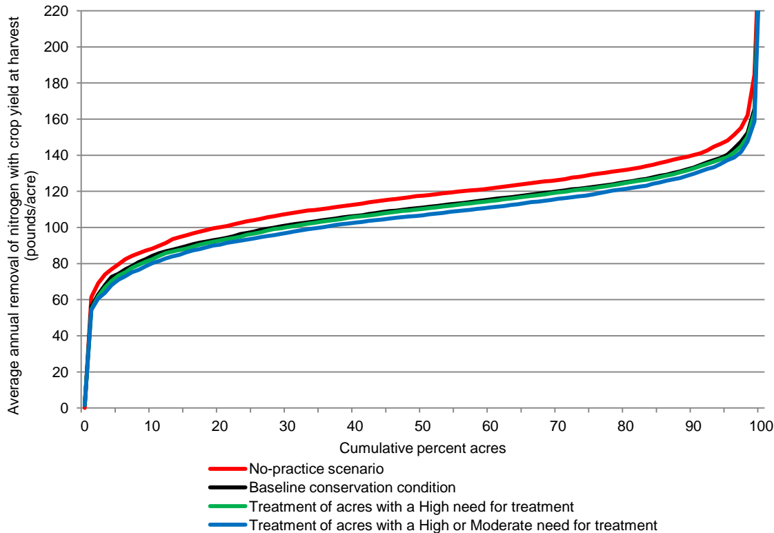
Figure 74. Estimates of average annual removal of nitrogen with crop yield at harvest for undertreated acres treated with water erosion control and nutrient management compared to the baseline conservation condition and the no-practice scenario, Upper Mississippi River Basin
