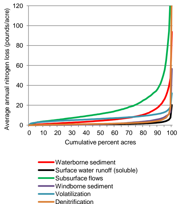
Figure 29. Cumulative distributions of average annual nitrogen lost through various loss pathways, Upper Mississippi River Basin, baseline conservation condition
