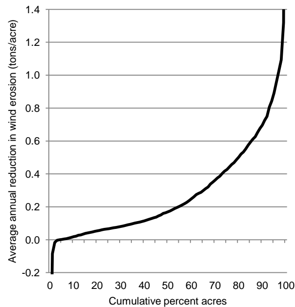
Figure 20 Estimates of average annual reduction in wind erosion due to the use of conservation practices on cropped acres in the Upper Mississippi River Basin
