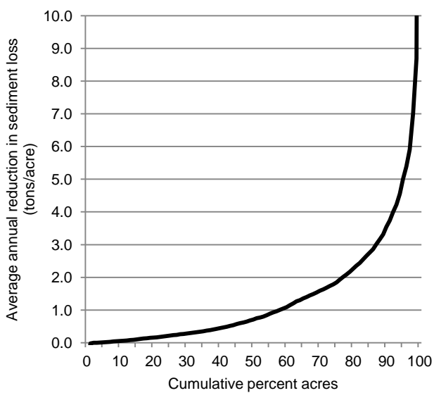
Figure 23. Estimates of average annual reduction in sediment loss due to the use of conservation practices on cropped acres in the Upper Mississippi River Basin
