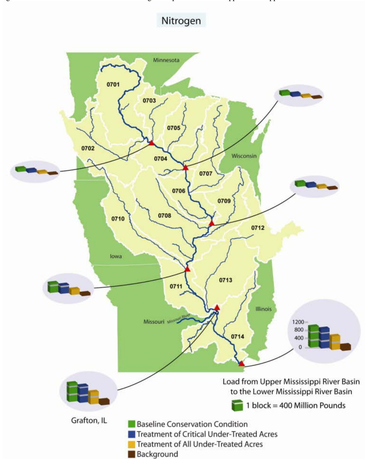
Figure 90. Estimates of average annual instream nitrogen loads* for the baseline conservation condition compared to two scenarios simulating additional erosion control and nutrient management practices for the Upper Mississippi River Basin
