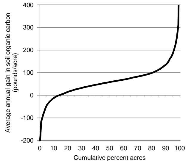
Figure 26. Estimates of average annual gain in soil organic carbon due to the use of conservation practices on cropped acres in the Upper Mississippi River Basin
