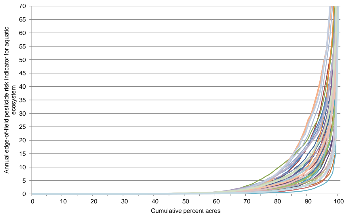
Figure 45. Distribution of annual values of the edge-of-field surface water pesticide risk indicator for aquatic ecosystems for each year of the 47-year model simulation, Upper Mississippi River Basin
