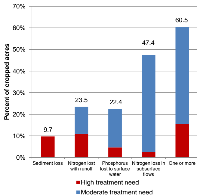
Figure 61. Percent of cropped acres that are undertreated in the Upper Mississippi River Basin, by resource concern
