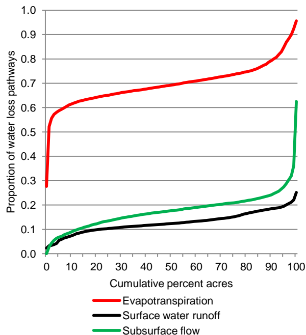
Figure 14. Cumulative distributions of the proportion of water lost through three loss pathways for cropped acres, Upper Mississippi River Basin
