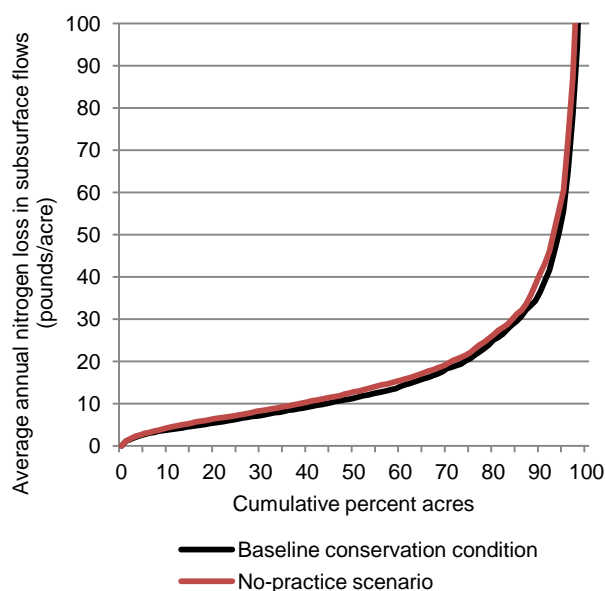
Figure 36. Estimates of average annual nitrogen loss in subsurface flows for cropped acres in the Upper Mississippi River Basin
