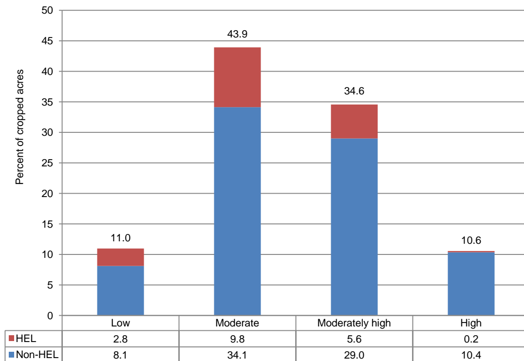
Figure 51. Percent of cropped acres at four conservation treatment levels for phosphorus runoff control in the baseline conservation condition, Upper Mississippi River Basin
