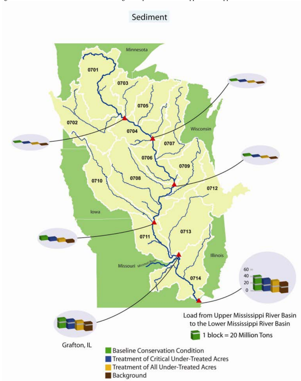
Figure 89. Estimates of average annual instream sediment loads* for the baseline conservation condition compared to two scenarios simulating additional erosion control and nutrient management practices for the Upper Mississippi River Basin
