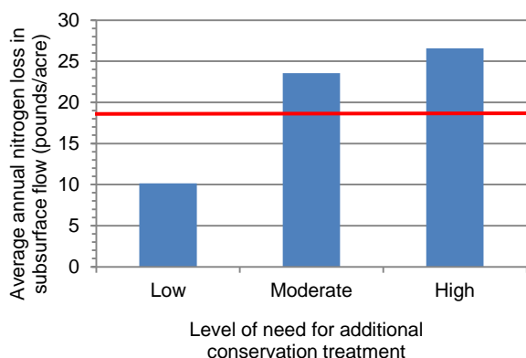
Figure 65. Average per-acre nitrogen loss in subsurface flow pathways for three levels of conservation treatment need for one or more resource concerns, Upper Mississippi River Basin
