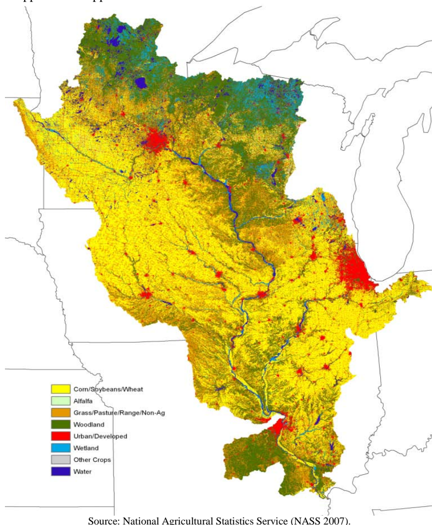
Figure 1. Land cover in the Upper Mississippi River Basin
