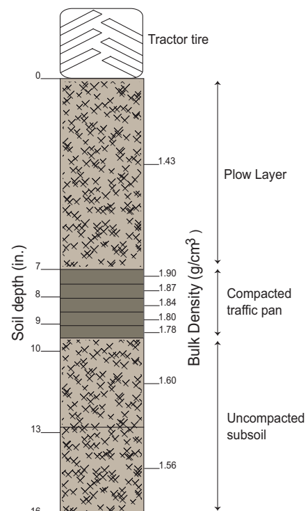
Figure 1. Tillage and heavy equipment traffic compacted soil below the plow layer of an Udult soil (Norfolk), inhibiting root penetration and water movement through the soil profile.
